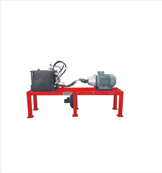
Electro-hydraulic drive
