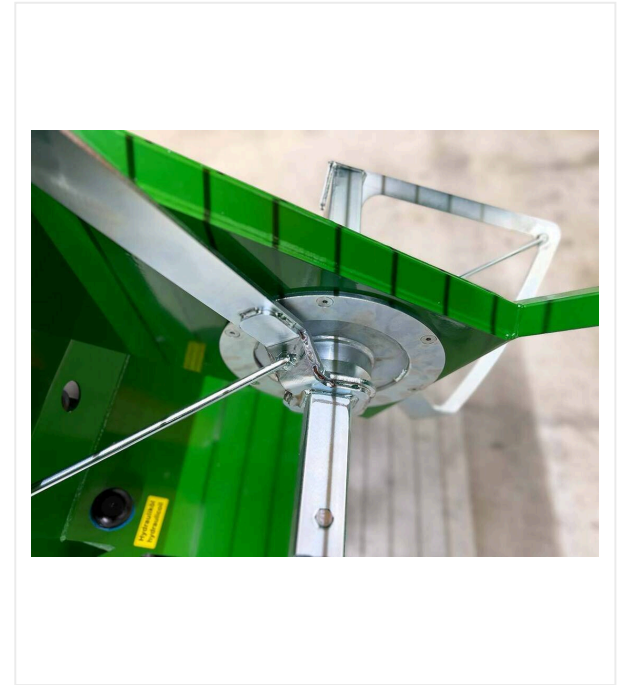
Mixing tool integrated in the mixing head, hydraulically liftable
