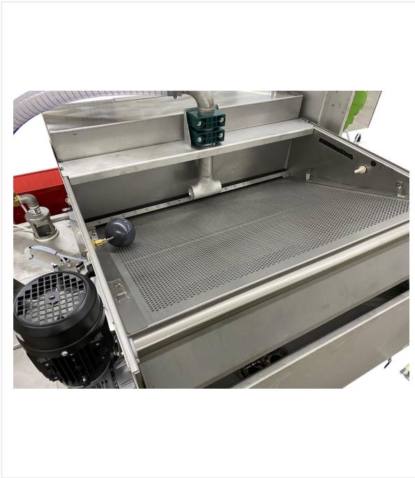
Belt filter with tear-resistant filter fleece (120 \mu\text{m} ) including collecting container with float switch
