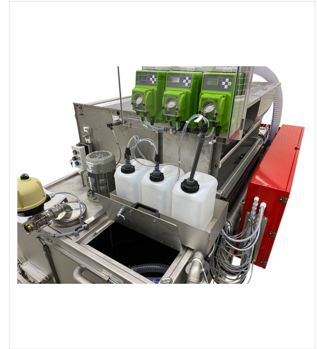
Storage tank and dosing station for flocculants, optionally cleaning agents etc.
