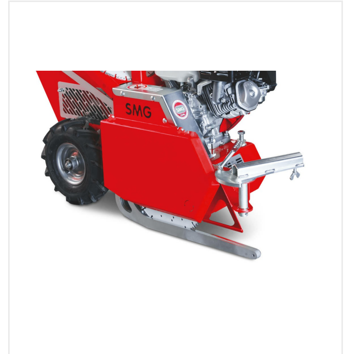
Sword, saw blade and 180° swiveling guide-chain
